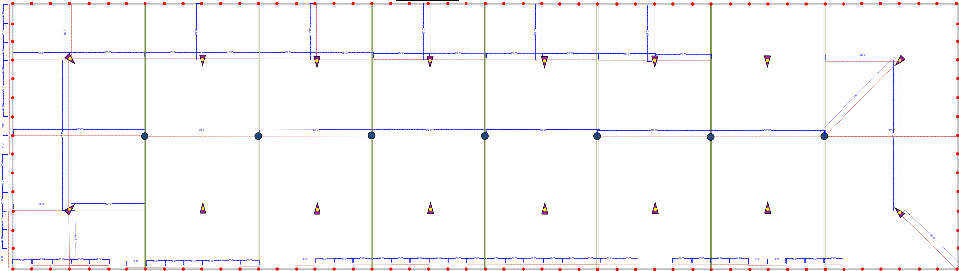
70' x 250' Pole Tent - Pole Placements
